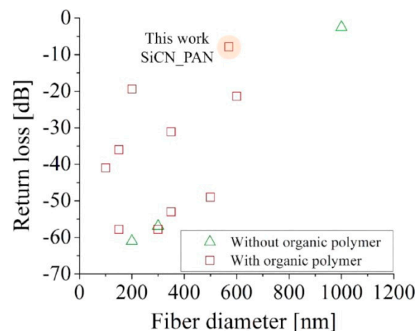
Figure 6. Relationship between diameter versus return loss of electrospun ceramic fibers from Si-based preceramic polymers. From [80], copyright (2022), with permission from Elsevier. “This work” refers to [84].
