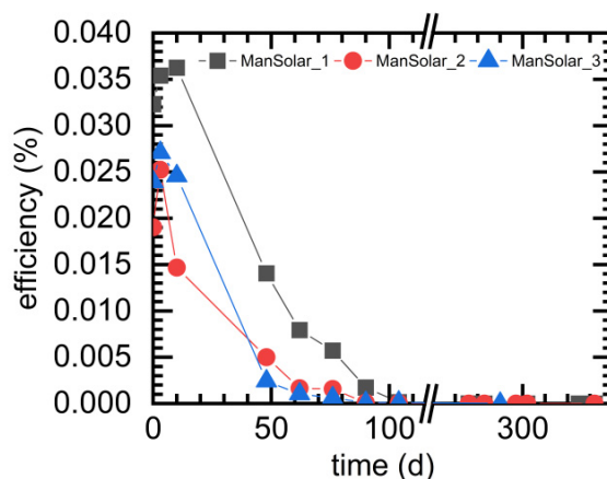
Figure 3. Efficiency of DSSCs produced with commercial fluid electrolyte, measured for approx. 1 year.
