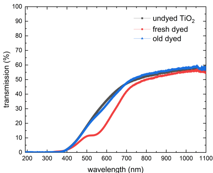
Figure 1. Transmission spectra of undyed TiO 2 on FTO coated glass, fresh and old dyed TiO 2 layers on FTO coated glass.
