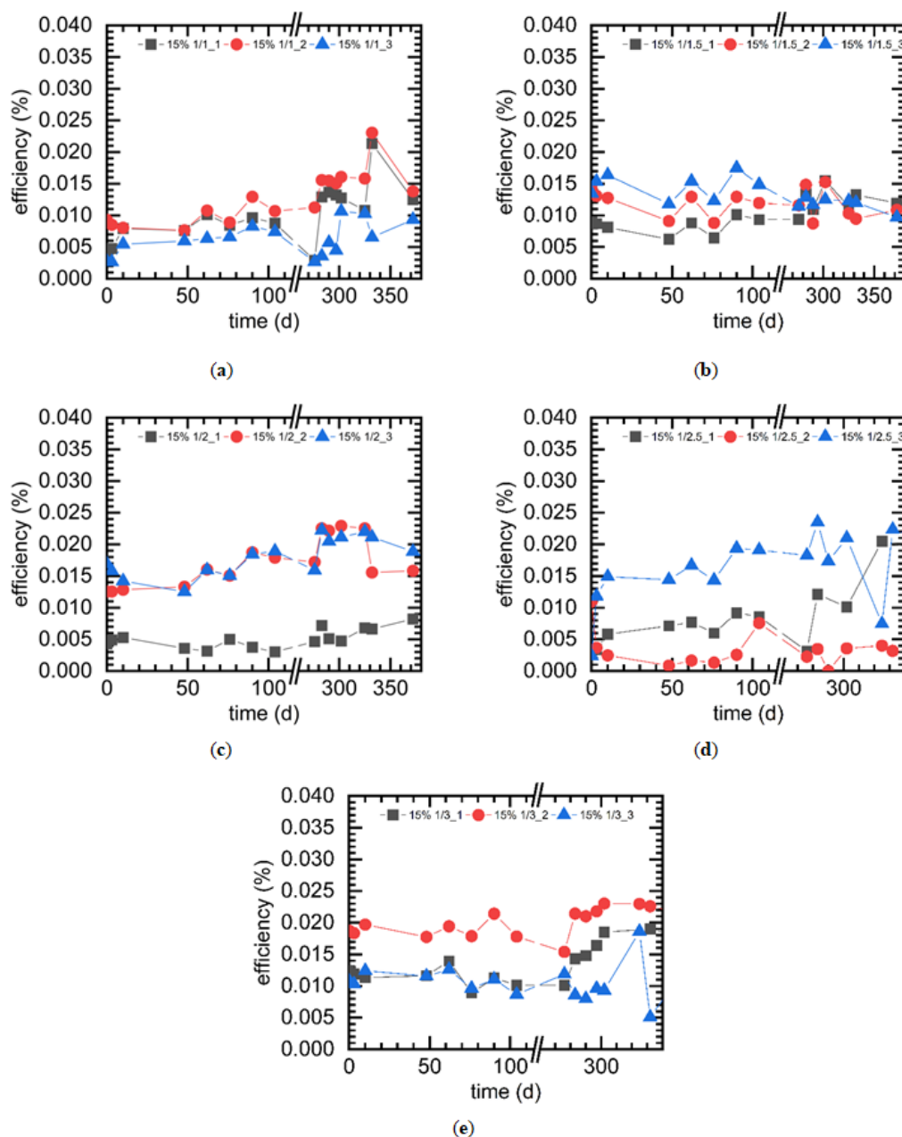
Figure 4. Efficiency of DSSCs produced with 15 wt% iodine and different iodine:potassium iodide mass ratios, measured for approx. 1 year: (a) 1:1; (b) 1:1.5; (c) 1:2; (d) 1:2.5; (e) 1:3.
