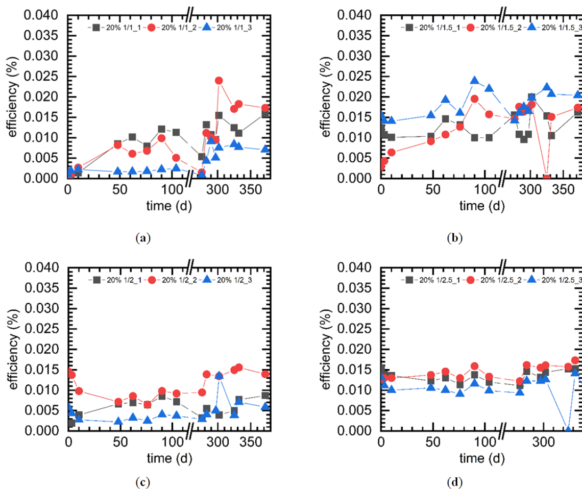
Figure 5. Efficiency of DSSCs produced with 20 wt% iodine and different iodine:potassium iodide mass ratios, measured for approx. 1 year: (a) 1:1; (b) 1:1.5; (c) 1:2; (d) 1:2.5.
