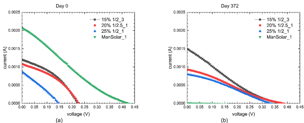
Figure 2. Current-voltage curves of exemplary DSSC with glycerol-based or commercial electrolyte: (a) measured directly after preparation (day 0); (b) measured at the end of the experiment (day 372).
