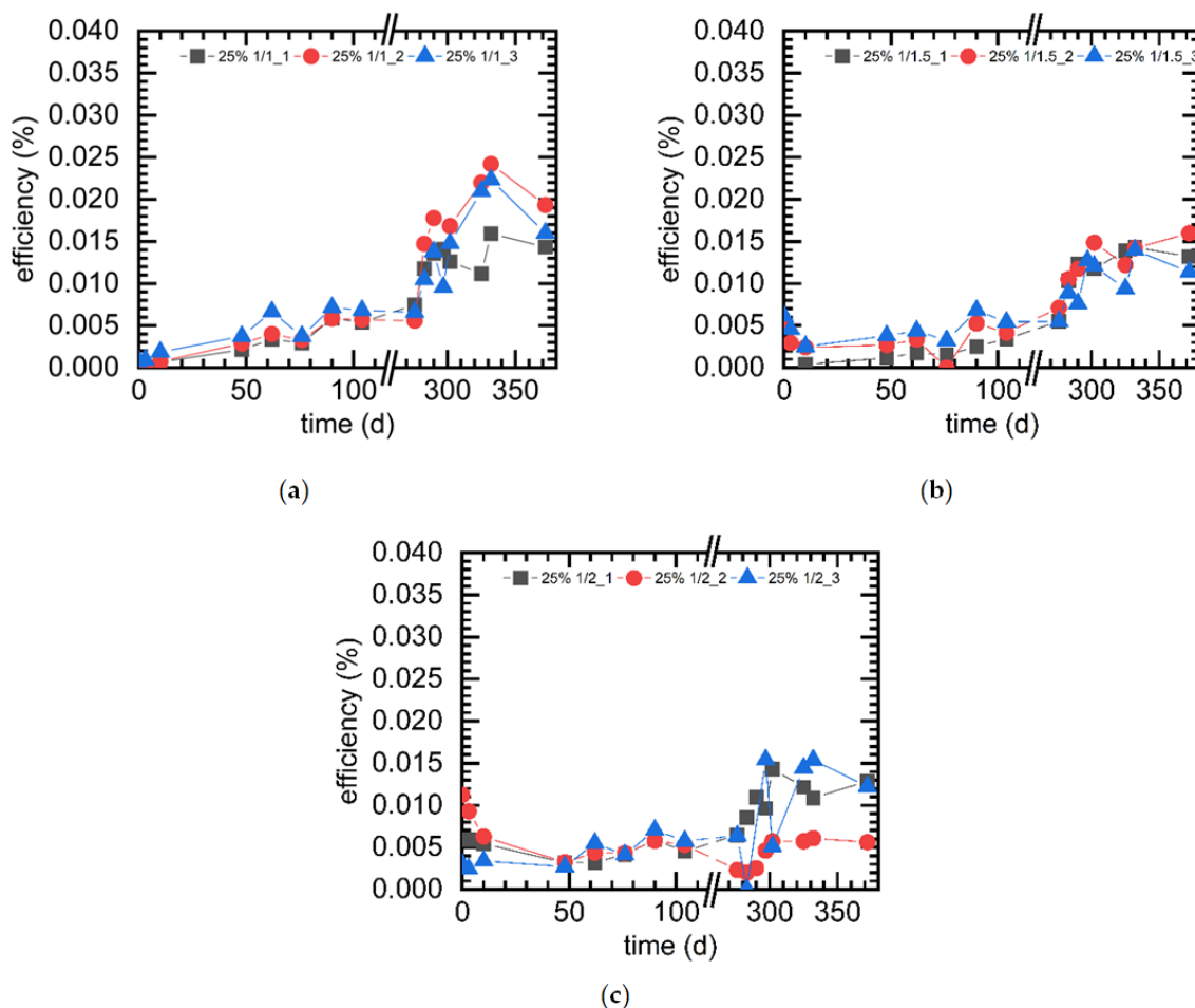
Figure 6. Efficiency of DSSCs produced with 25 wt% iodine and different iodine:potassium iodide mass ratios, measured for approx. 1 year: (a) 1:1; (b) 1:1.5; (c) 1:2.
