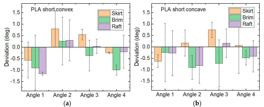
Figure 5. Angle deviations of short PLA samples: (a) convex; (b) concave.
