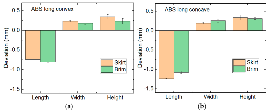
Figure 8. Length deviations of long ABS samples: (a) convex; (b) concave.
