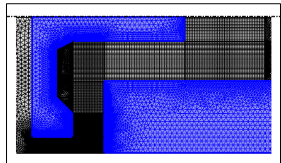
Figure 4: Mesh refinement
