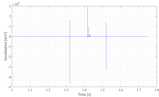
Figure 10: Time-Acceleration diagram
