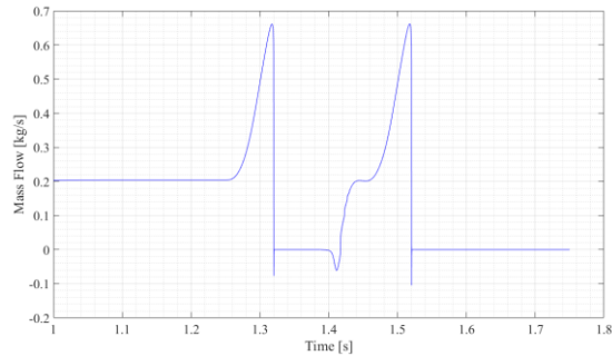
Figure 11: Time-Mass flow diagram
